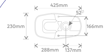
Vista Base
