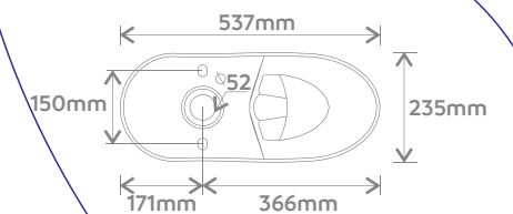
Vista Base
