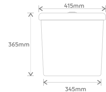
Vista Frontal
